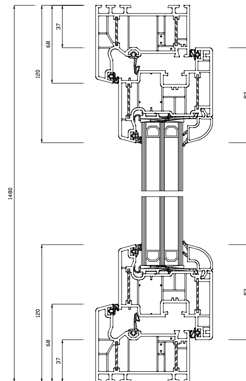
Øez S1(5:1)
